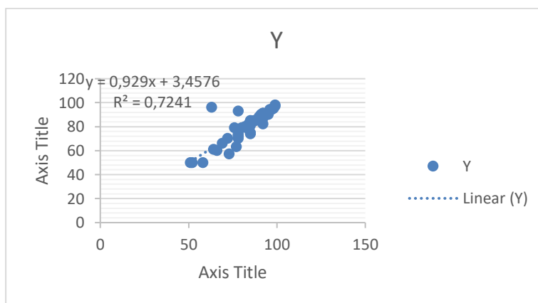
Figure 5 Regression Direction Test
